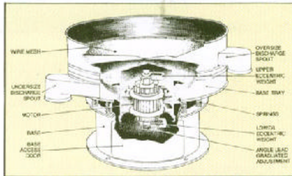
Cross Sectional View of a Single Deck Machine
